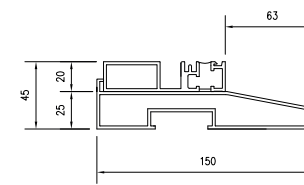
Low Threshold with 150mm Cill
