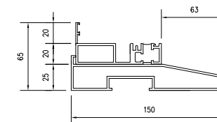
Low Threshold with Rebate & 150mm Cill
