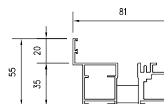
Standard Threshold - No Cill
