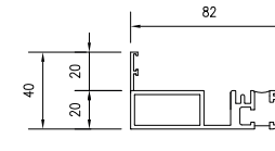
Low Threshold with Rebate - No Cill
